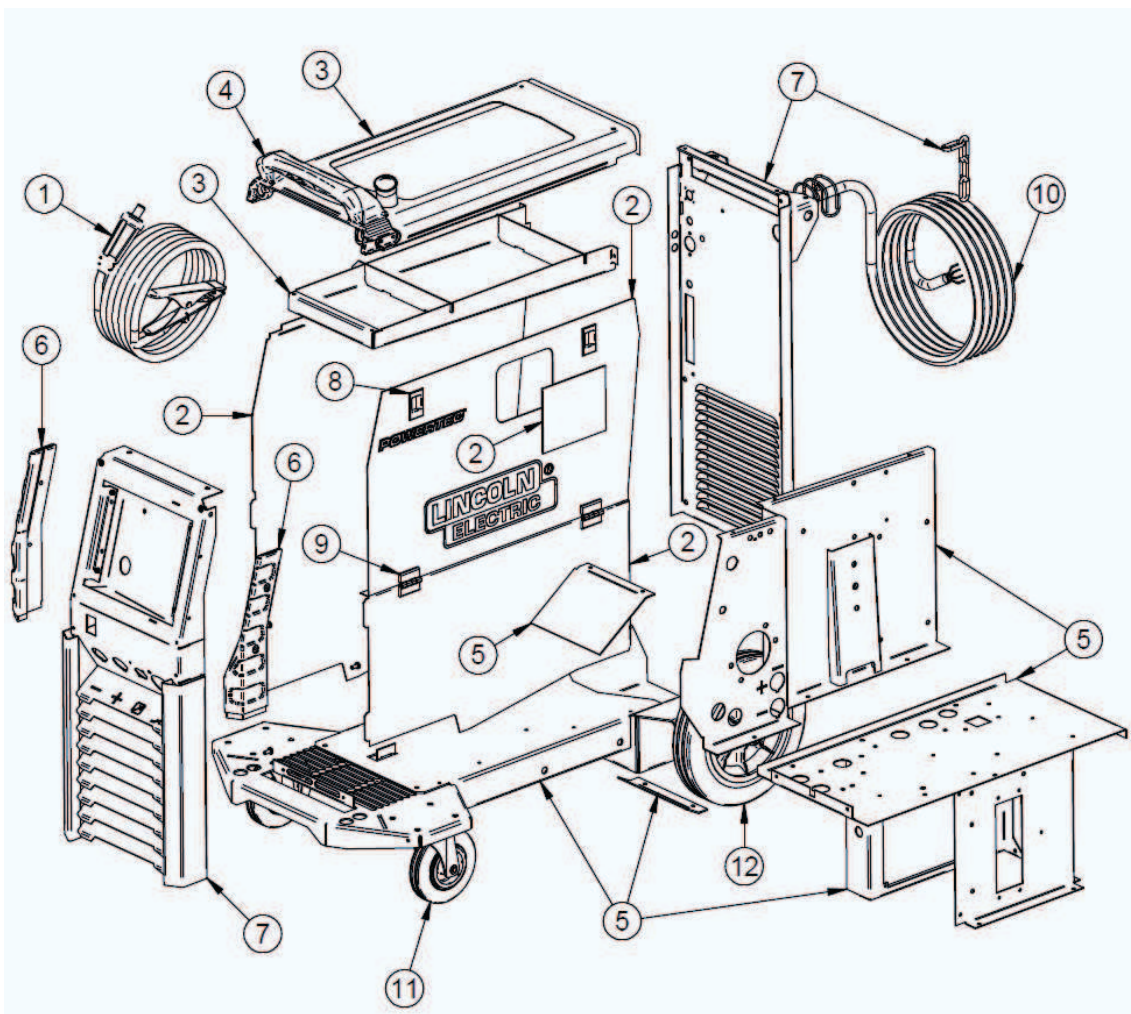
Figure A. Powertec i250C/i320C STD/ADV Machine Assembly
