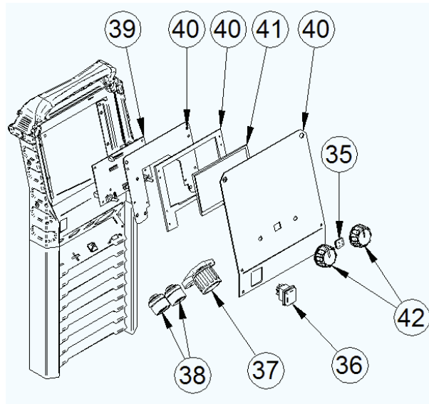
Figure E: Powertec i250C/i320C ADV Front Assembly
