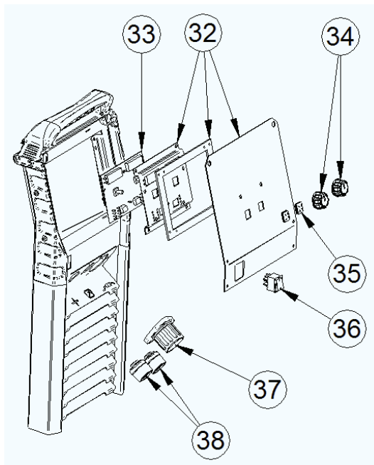
Figure D: Powertec i250C/i320C STD Front Assembly
